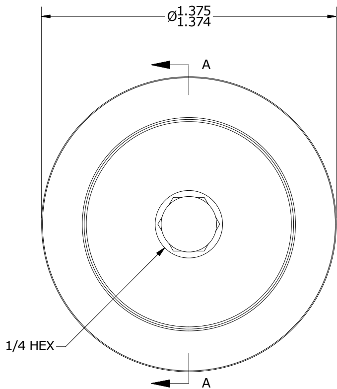
END VIEW SCALE 2.25 : 1
