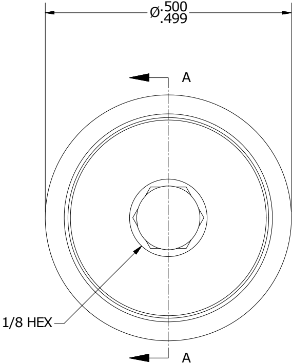
END VIEW SCALE 5 : 1
